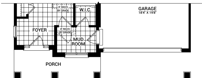
MAIN FLOOR PLAN B
