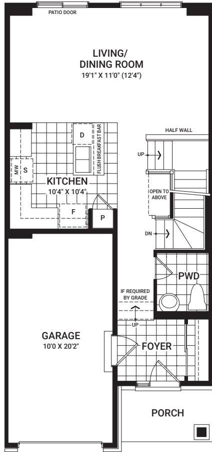
MAIN FLOOR
