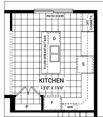
OPTIONAL KITCHEN LAYOUT A
