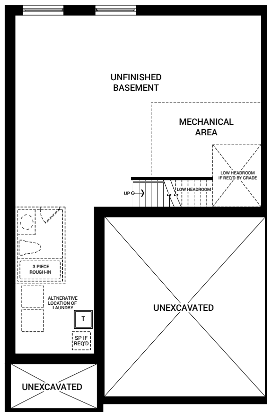
BASEMENT PLAN A, C & D
