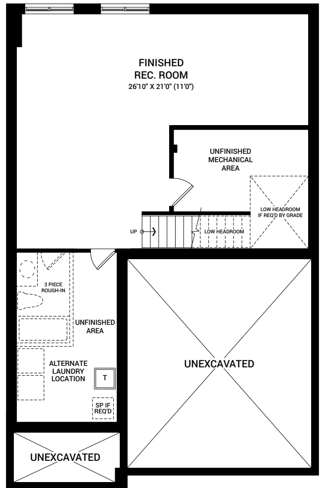
OPTIONAL FINISHED BASEMENT REC. ROOM
